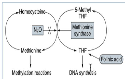
Fig. 17.3 Pathway showing the inhibition of methionine synthase by nitrous oxide (N 2 O) and its potential metabolic consequences (e.g., decreased DNA synthesis and impaired methylation reactions). THF, Tetrahydrofolate. (Courtesy of M. Fujinaga, Palo Alto, CA.)
